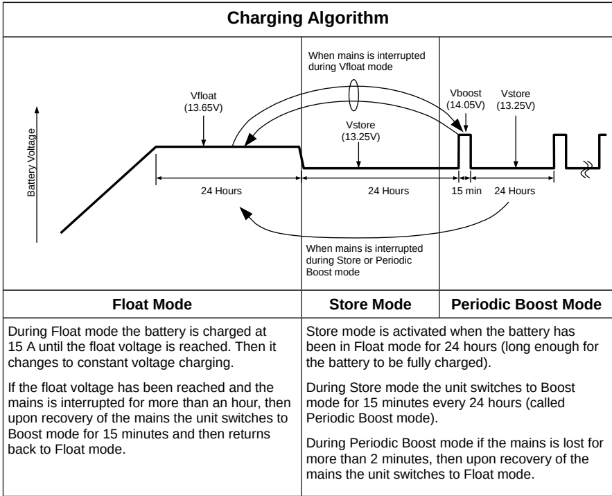
Figure 6: Charging Algorithm
